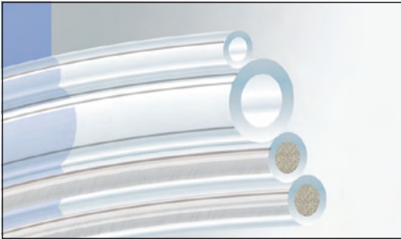
Thermo-bonded paratube with encapsulated silver wires
